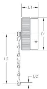
CIRTF
