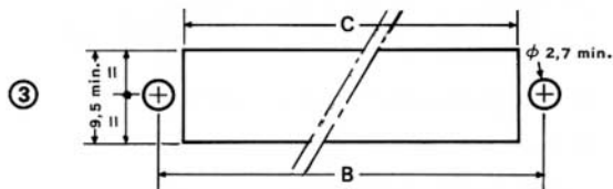
Fig. 3: for receptacles and screwlock sockets without brackets max. panel thickness: 3.2 mm
