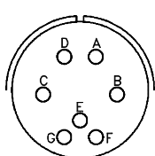
ARRANGEMENT 22-33 CONTACT SIZE 16 SERVICE RATING A,B,C,D=D ; E,F,G=A
