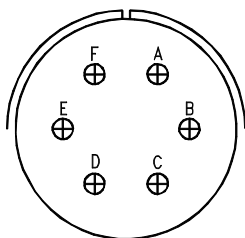
ARRANGEMENT 40-A6 CONTACT SIZE 16 SERVICE RATING B
